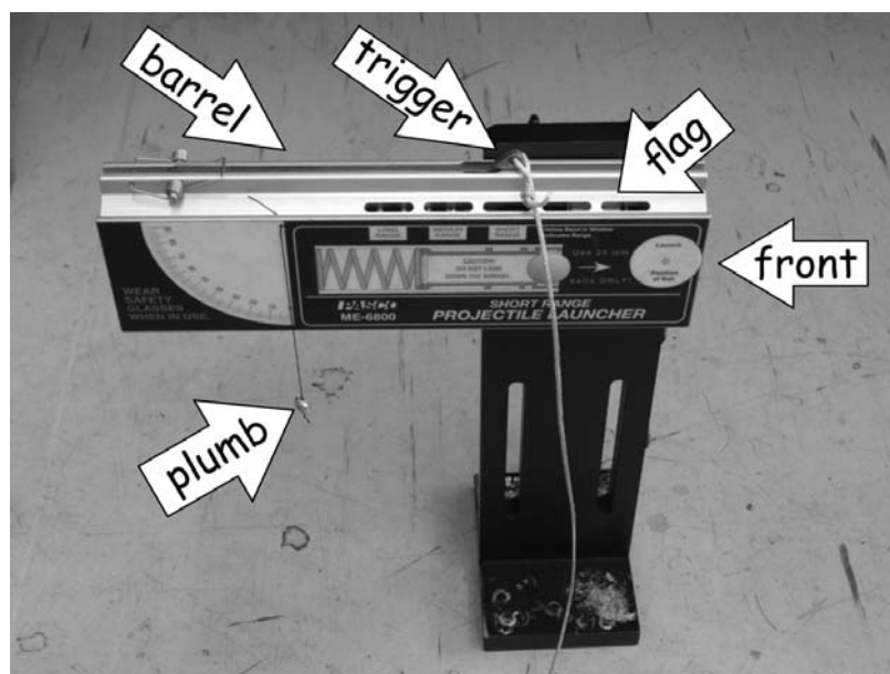
Fig. 4 The projectile launcher - the two fastening bolts is on the other side of the launcher.
